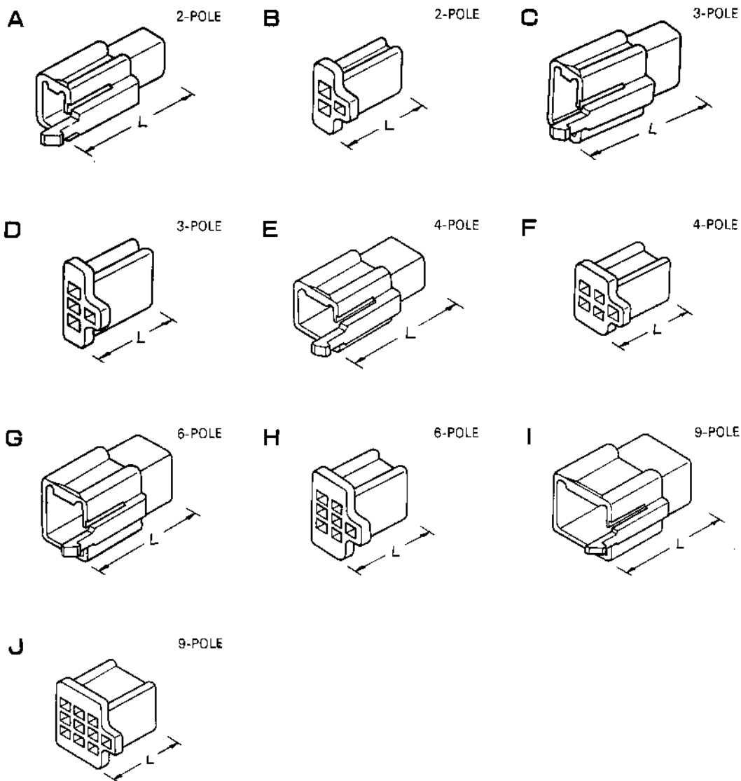
.110 Series Housings(with lock) Specification
